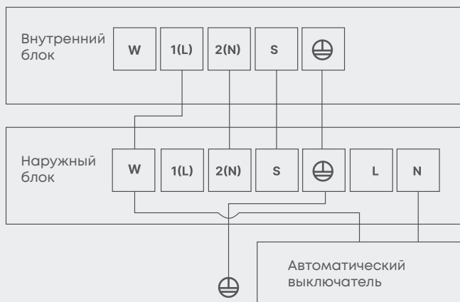
MDSBI-09-24HRFN8
